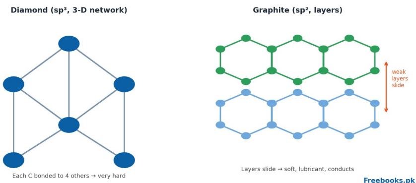
Figure 3.3 — Diamond (rigid 3-D network) versus graphite (sliding layers).
