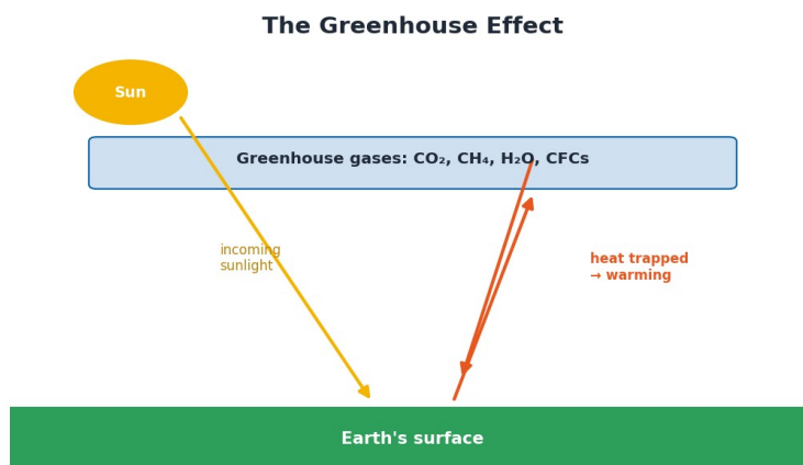
Figure 16.4 — The greenhouse effect.
