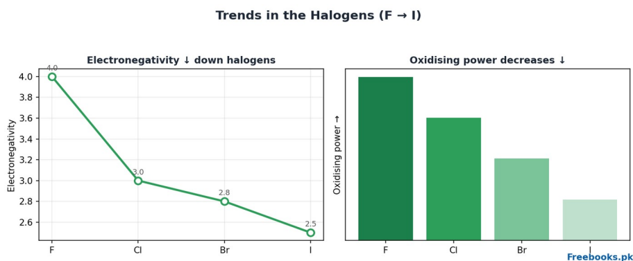
Diagram 1 — Halogen trends (F → I).
