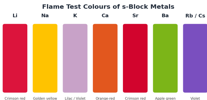
Diagram 1 — Flame test colours.
