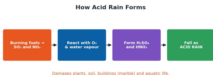
Figure 16.3 — Formation of acid rain.
