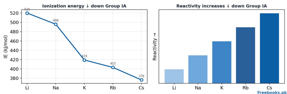
Figure 2.2 — Down Group IA, ionization energy decreases and reactivity increases.
