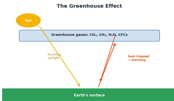
Diagram 1 — The greenhouse effect.
