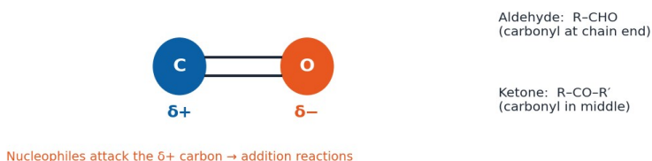
Diagram 1 — The carbonyl group.
